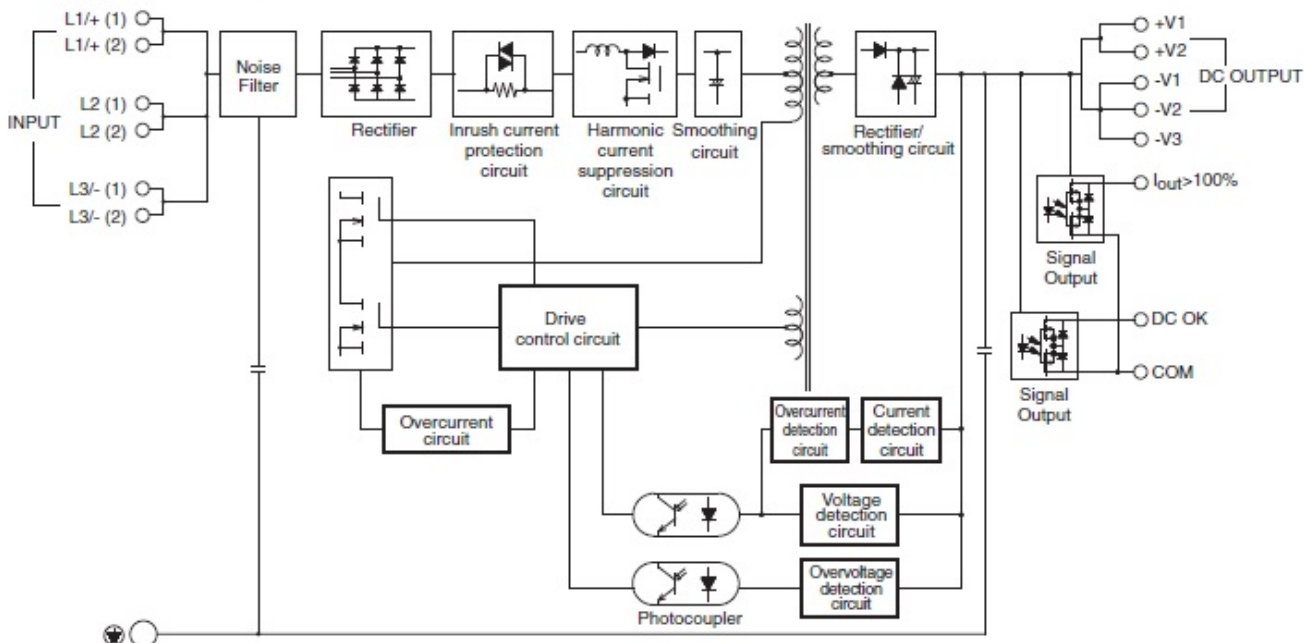
S8VK-WA24024 (240 W)
