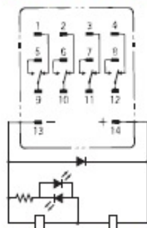
(Coil has polarity)
