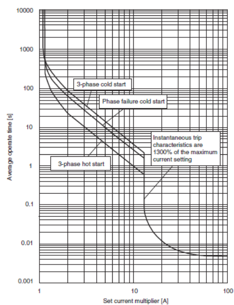
Average values of operating characteristics (reference values)
