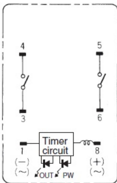
Bottom View
