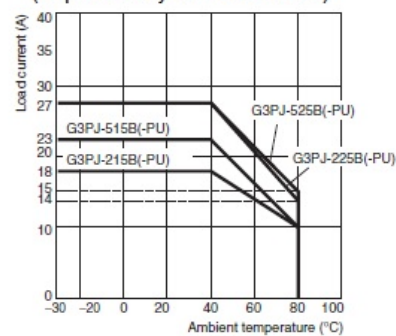
Separate Mounting (Separated by 10 mm or More)
