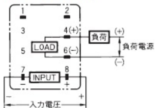
端子配置/内部接続 (BOTTOM VIEW)
