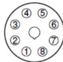
端子配置 (BOTTOM VIEW)
