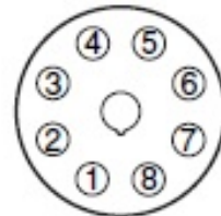
端子配置 (BOTTOM VIEW)
