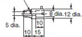
Details of mounting bracket
