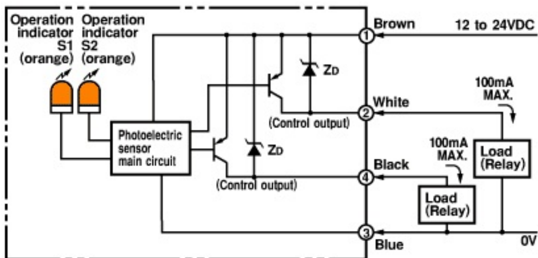
M8 Connector Pin Arrangement
