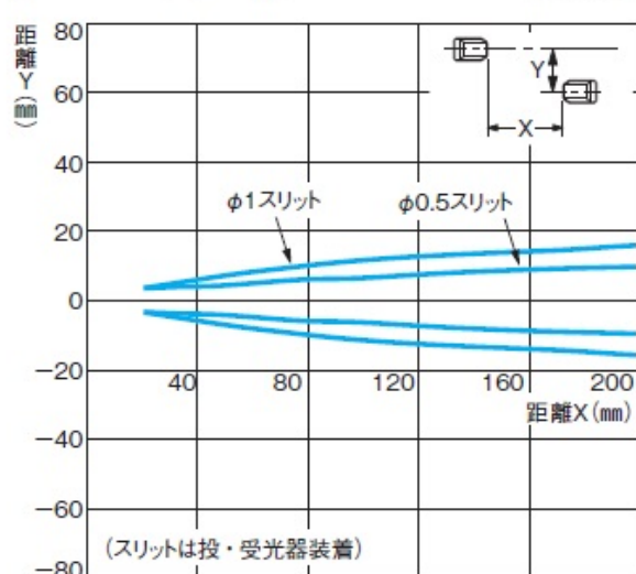
形E3T-ST1□+形E39-S63 形E3T-ST1□M+形E39-S76A/S76B (拡大図)
