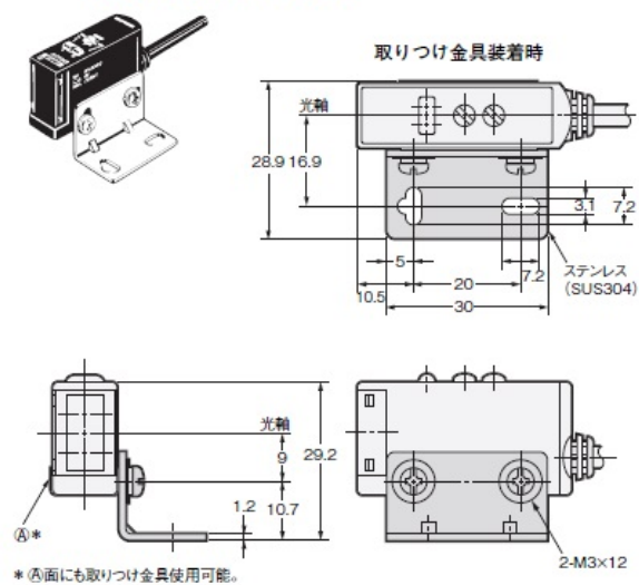
形E3S-AD11/12/13/21/22/23 -AD31/32/33/41/42/43
