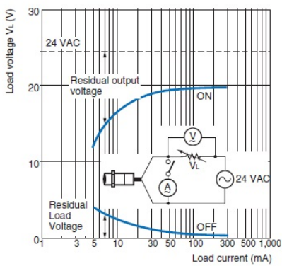
E2FQ-X□Y1 at 24 VAC
