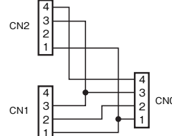
形XS2R-D426-82
