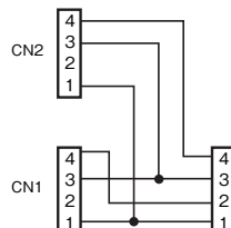
形XS2R-D426-81
