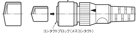
形XS2Z-15
