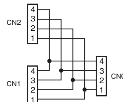
形XS2R-D426-82
