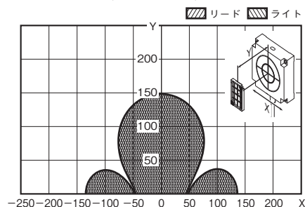
形V680-HS63(背面：金属) &amp; 形V680S-D2KF68M(RFタグ縦向き)
