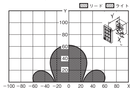
形V680-HS65(背面：金属) &amp; 形V680S-D2KF68M(RFタグ縦向き)
