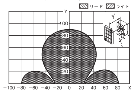
形V680-HS65(背面：金属) &amp; 形V680S-D2KF68(RFタグ縦向き)
