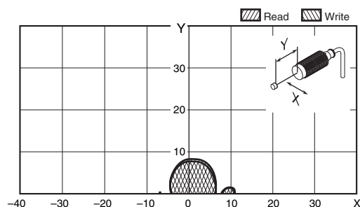
V680-HS61 (mounted on non-metallic material) & V680-D1KP53M (embedded in metallic surface: steel)
