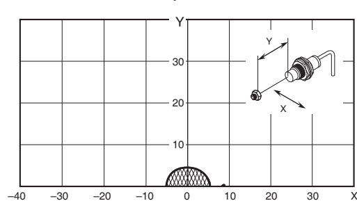
V680-HS52 (embedded in non-metallic material) & V680-D2KF52M-BT01 (mounted in metal/non-metallic material)
