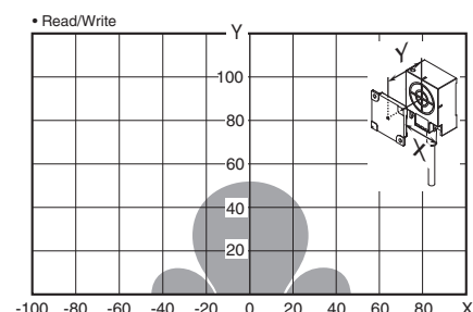
V680-HS52 (embedded on non-metallic material) & V680S-D8KF67M (mounted on metallic surface: steel)
