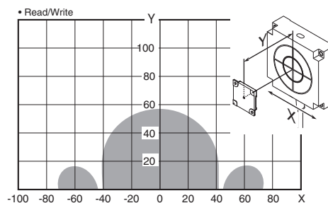
V680-HS63 (mounted on non-metallic material) & V680S-D8KF68 (Tag direction: Vertical)
