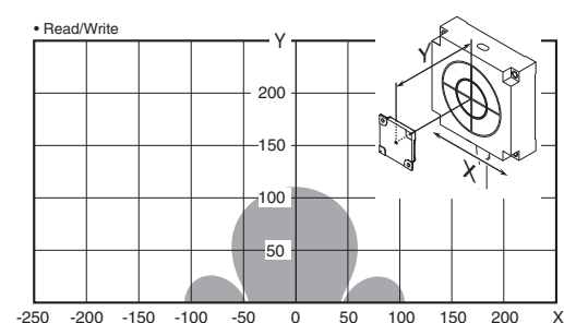
V680-HS61 (mounted on non-metallic material) & V680S-D8KF67M (mounted on metallic surface: steel)
