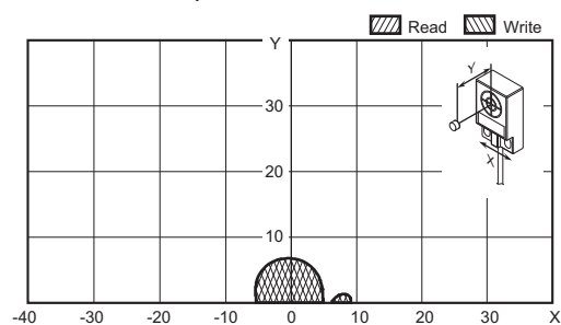
V680-HS52 (embedded in Non-Metal) & V680S-D2KF67 (mounted on non-metallic material)
