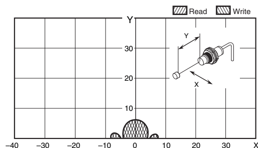
V680-HS61 (mounted on non-metallic material) & V680-D2KF52M (embedded in metallic surface: steel)
