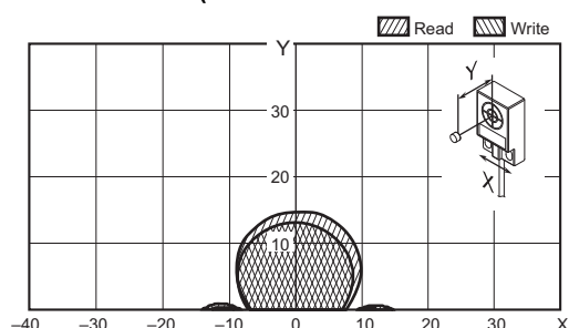
V680-HS52 (embedded in non-metallic material) & V680-D1KP54T (mounted on non-metallic material)
