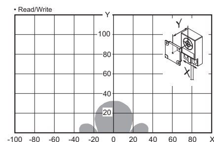
V680-HS65 (mounted on metallic material) & V680S-D8KF67M (mounted on metallic surface: steel)
