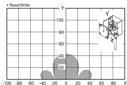
V680-HS63 (mounted on non-metallic material) & V680S-D8KF68 (Tag direction: Horizontal)
