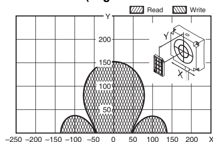
V680-H01-V2 (with Non-Metal on Back Surface) & V680S-DKF68 (Tag direction: Vertical)
