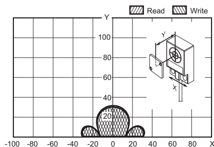
V680-HS61 (embedded in non-metallic material) & V680-D1KP66MT (mounted on metallic surface: steel)
