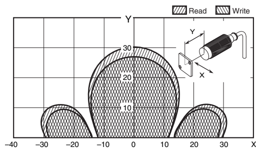
V680-HS52 (embedded in non-metallic material) & V680-D1KP66MT (mounted on metallic surface: steel)
