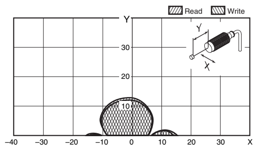
V680-HS61 (mounted on non-metallic material) & V680-D1KP53M (embedded in non-metallic material)
