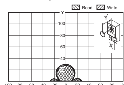
V680-HS65 (mounted on metallic material) & V680-D1KP54T (mounted on non-metallic material)
