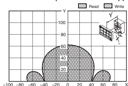
V680-HS65 (with Metal on Back Surface) & V680S-D2KF68M (Metal on back: Steel) (Tag direction: Horizontal) V680-HS65 (with Metal on Back Surface) & V680S-D2KF68M (Metal on back: Steel) (Tag direction: Vertical)
