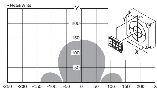
V680-H01-V2 (mounted on non-metallic material) & V680S-D8KF68 (Tag direction: Horizontal)
