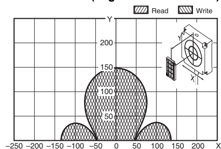
V680-HS63 (with Metal on Back Surface) & V680S-D2KF68M (Metal on back: Steel) (Tag direction: Horizontal) V680-HS63 (with Metal on Back Surface) & V680S-D2KF68M (Metal on back: Steel) (Tag direction: Vertical)
