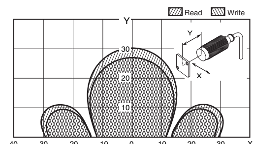
V680-HS63 (mounted on non-metallic material) & V680-D1KP66MT (mounted on metallic surface: steel)
