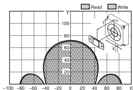
V680-HS52 (embedded in non-metallic material) & V680-D1KP66MT (mounted on metallic surface: steel)
