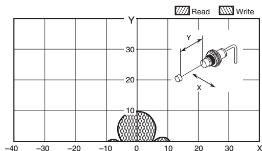
V680-HS61 (mounted on non-metallic material) & V680-D2KF52M (embedded in non-metallic material)
