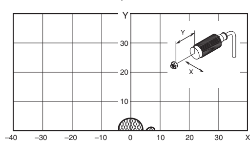
V680-HS51 (embedded in metallic material) & V680-D2KF52M-BT01 (mounted in metal/non-metallic material)
