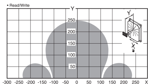
V680-H01-V2 (mounted on non-metallic material) & V680S-D8KF68 (Tag direction: Horizontal)
