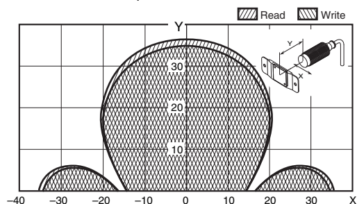
V680-HS65 (mounted on metallic material) & V680-D1KP66T-SP (mounted on non-metallic material)
