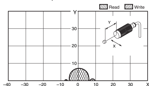
V680-HS52 (embedded in non-metallic material) & V680-D2KF52M (embedded in metallic surface: steel)
