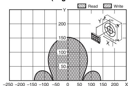
V680-H01-V2 (with Non-Metal on Back Surface) & V680S-DKF68 (Tag direction: Horizontal)
