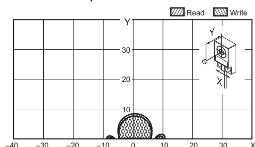
V680-HS61 (mounted on non-metallic material) & V680-D1KP54T (mounted on non-metallic material)
