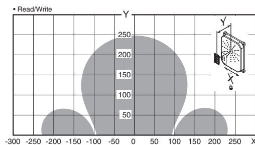
V680-H01-V2 (mounted on non-metallic material) & V680S-D8KF68 (Tag direction: Vertical)
