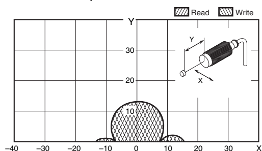
V680-HS52 (embedded in non-metallic material) & V680-D2KF52M (embedded in non-metallic material)
