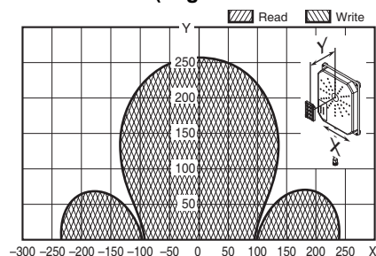
V680-HS63 (with Metal on Back Surface) & V680S-DKF68 (Metal on back: Steel) (Tag direction: Vertical)
