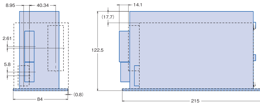
形S8VM-600□□+形S82Y-VM60S
