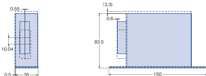
形S8VM-050□□+形S82Y-VM10B
