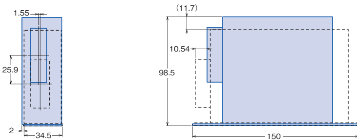
形S8VM-050□□+形S82Y-VM10B
