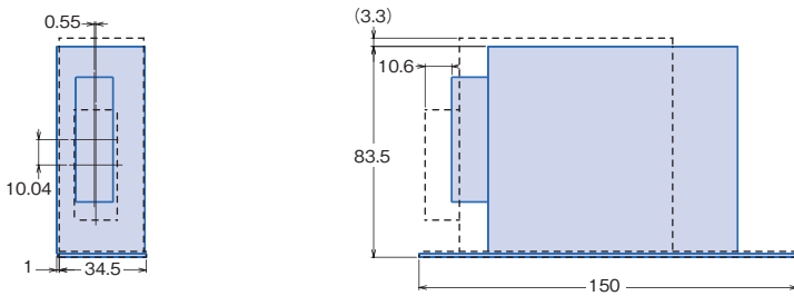
形S8VM-030□□+形S82Y-VM10B
