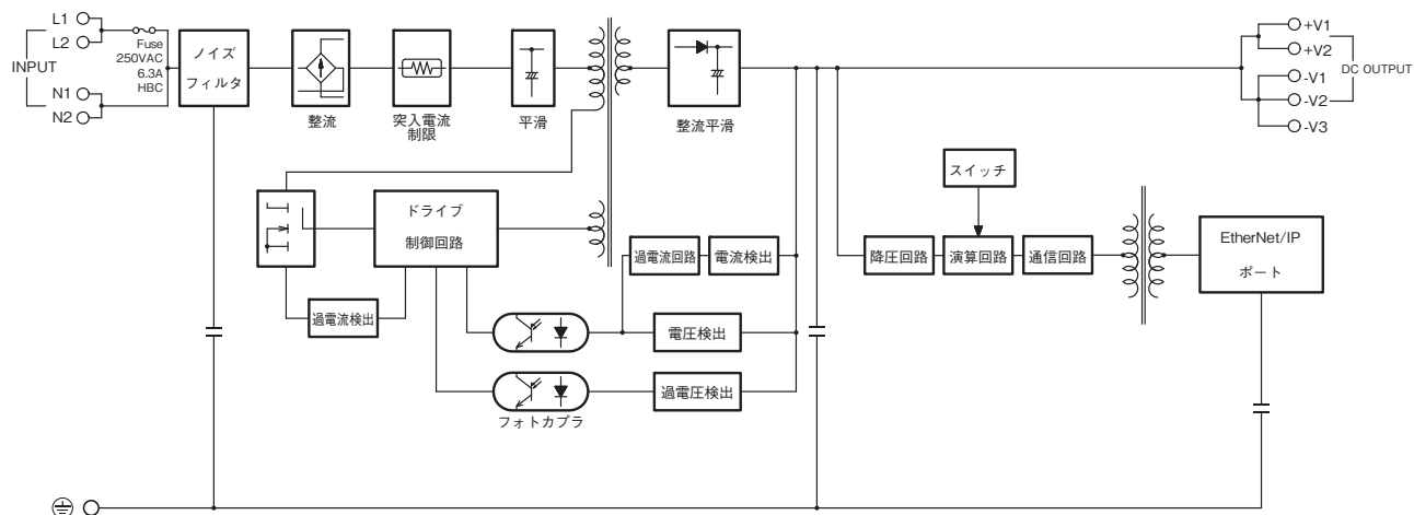
形S8VK-X09024□-EIP
