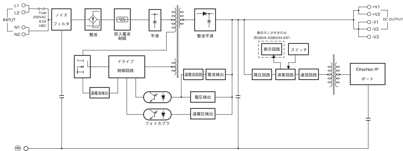
形S8VK-X12024□-EIP
