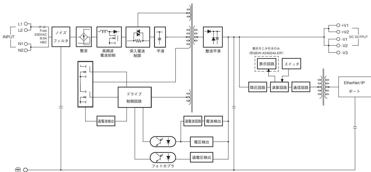
形S8VK-X48024□-EIP
