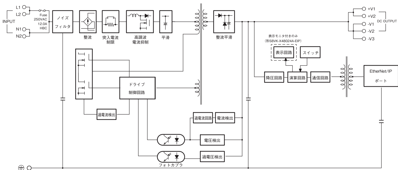
形S8VK-X48024□-EIP
