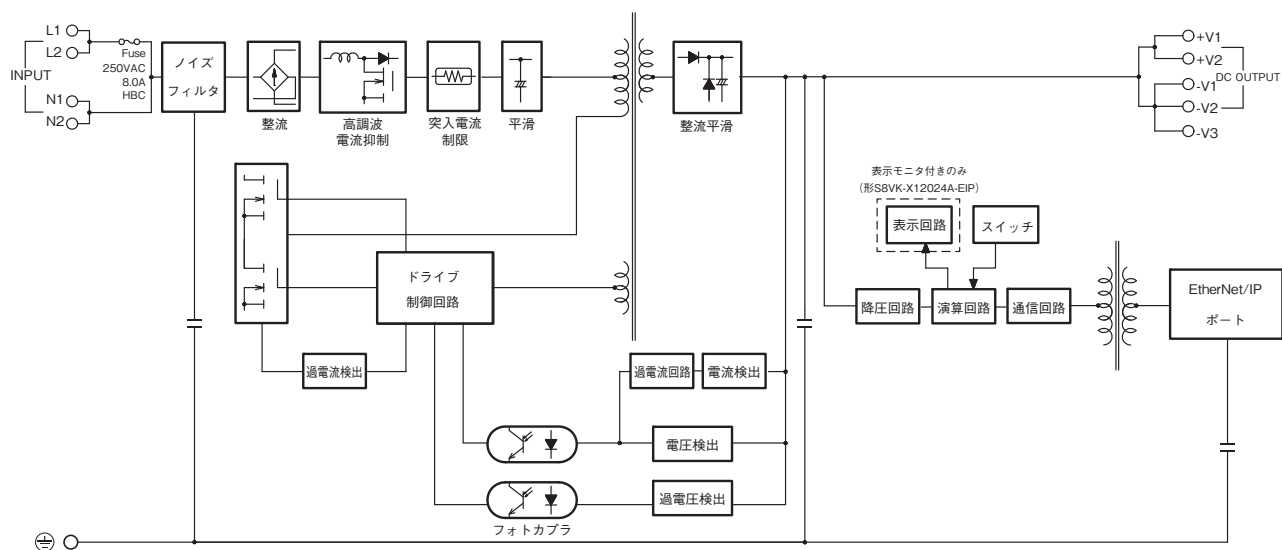
形S8VK-X12024□-EIP
