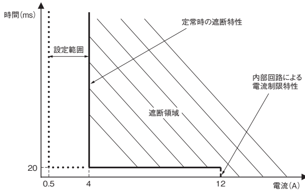
形S8M-CP04/形S8M-CP04-R
