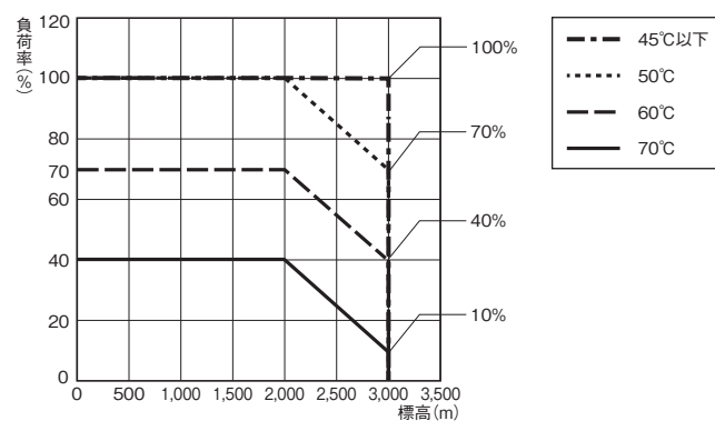
300W/600W
