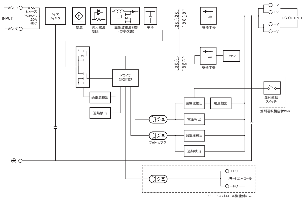
形S8FS-G600□□□ (600W)
