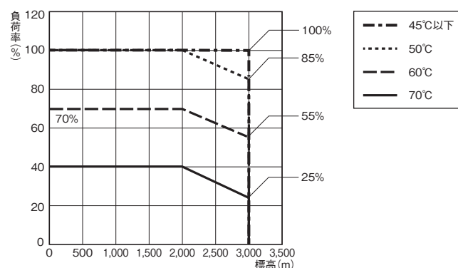
15W/30W/50W/100W/150W (AC入力時)
