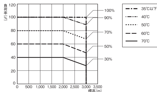
15W/30W/50W/100W/150W (DC入力時)
