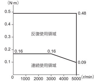
形R88M-G05030H
