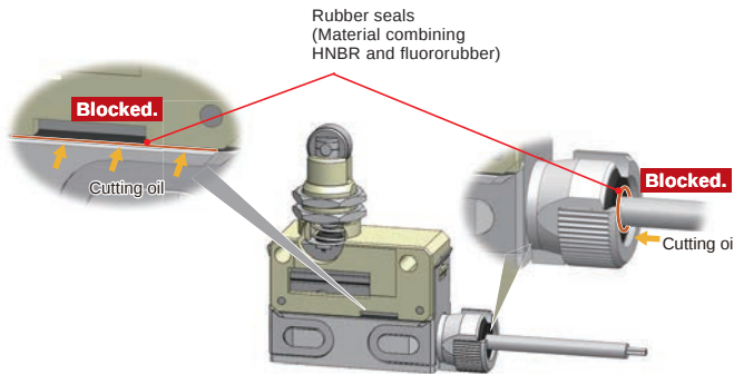
Figure 2. Terminal Section Protective Structure
