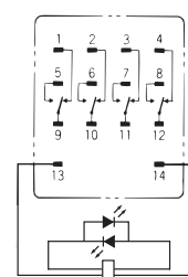
形MY4ZN-CBG (AC仕様)
