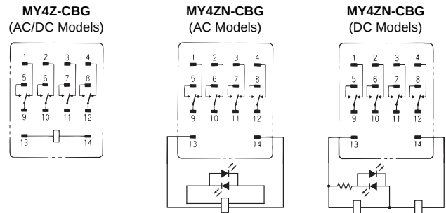
Terminal Arrangement/Internal Connection Diagram (Bottom View)
