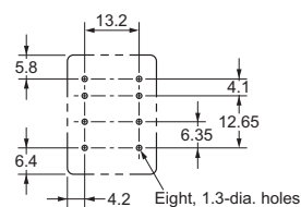
Mounting Hole and PCB Dimensions
