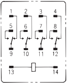
Terminal Arrangement/Internal Connection Diagram (Bottom View) MY4Z (AC/DC Models)
