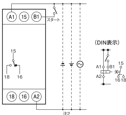
形H3DS-ML
