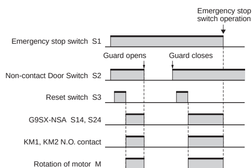
Timing chart
