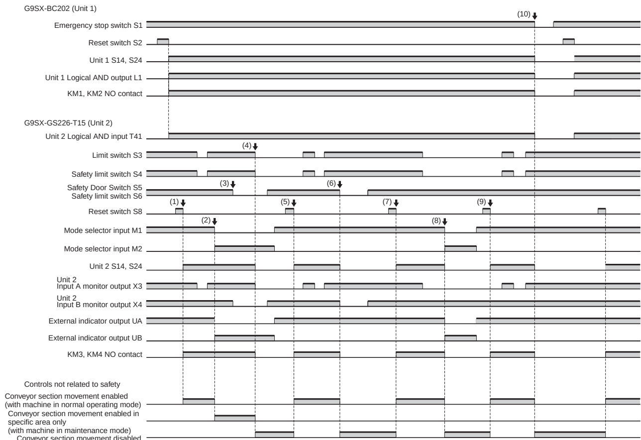
Timing Chart 2
