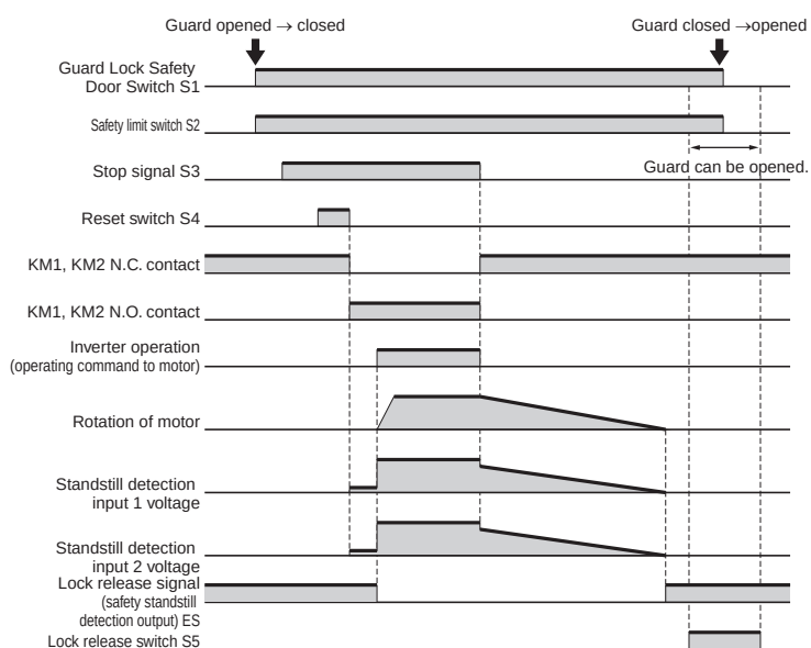
Timing Chart
