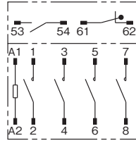
形G7Z-3A1B-11Z-R
