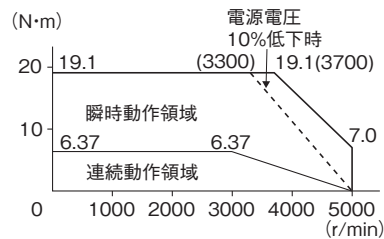
・形R88M-K2K030H/T (2kW)
