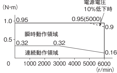
・形R88M-K75030H/T (750W)
