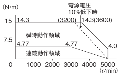
・形R88M-K1K530H/T (1.5kW)
