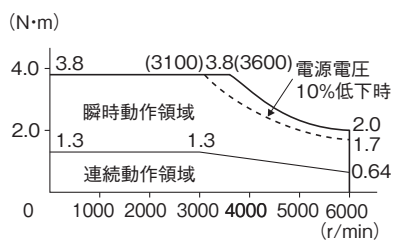
・形R88M-K40030H/T(400W)
