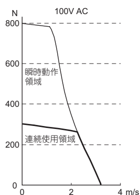
形R88L-EC-FW-1112
