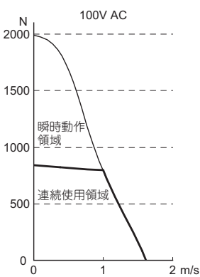
形R88L-EC-FW-1115
