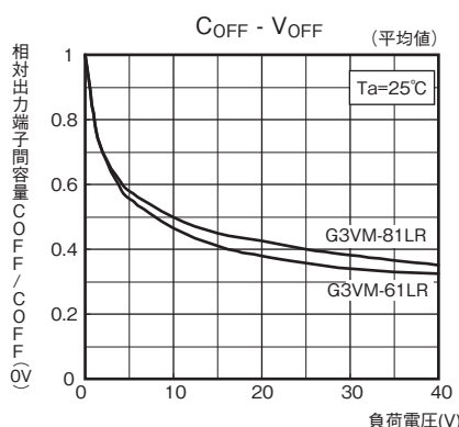
●相対出力端子間容量－負荷電圧 形G3VM-61LR/81LR
