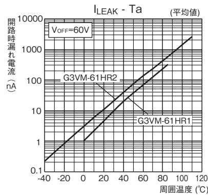
●開路時漏れ電流－周囲温度 形G3VM-61HR1/61HR2
