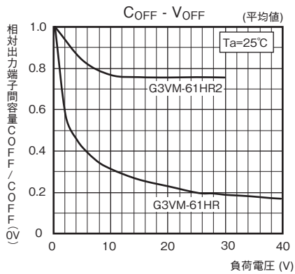
●相対出力端子間容量－負荷電圧 形G3VM-61HR/61HR2
