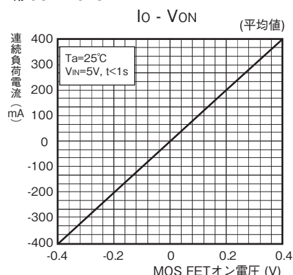
形G3VM-61UV
