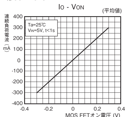
形G3VM-51UV
