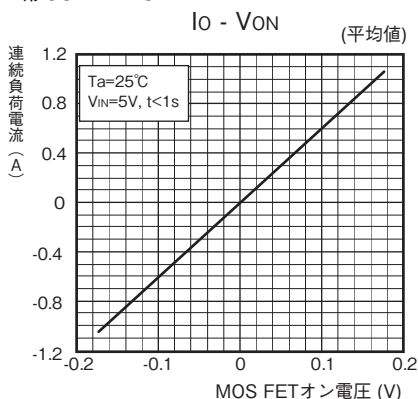
形G3VM-21UV11
