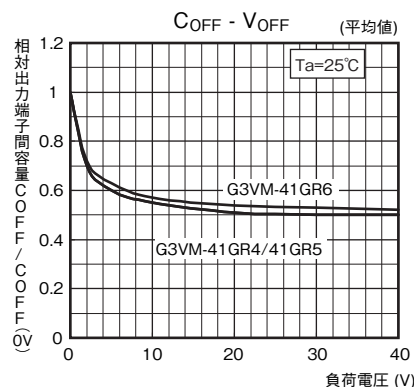
形G3VM-41GR6/41GR4/41GR5
