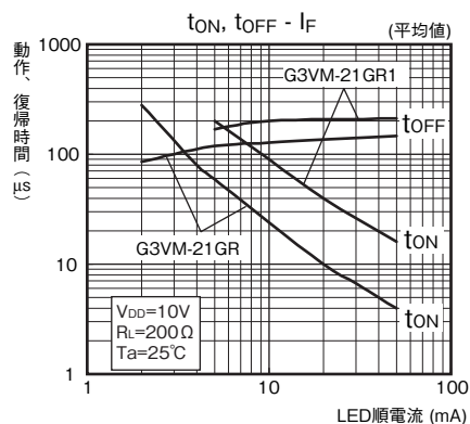
形G3VM-21GR/21GR1
