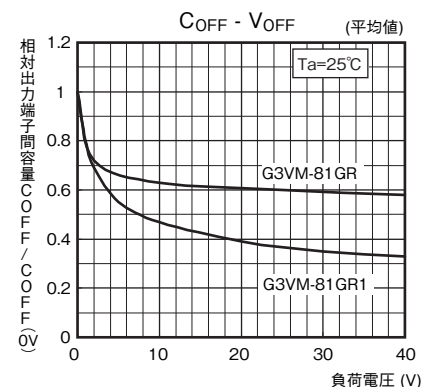
形G3VM-81GR/81GR1
