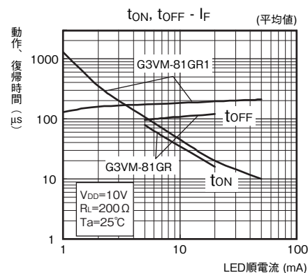
形G3VM-81GR/81GR1
