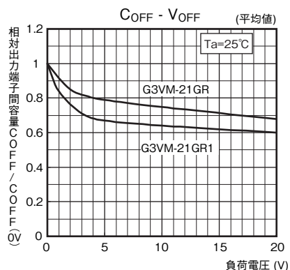
形G3VM-21GR/21GR1
