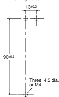
Mounting Holes
