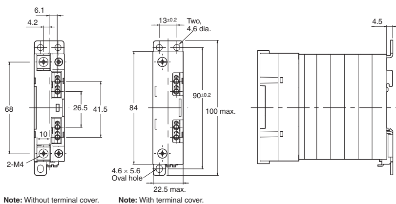
Mounting Holes
