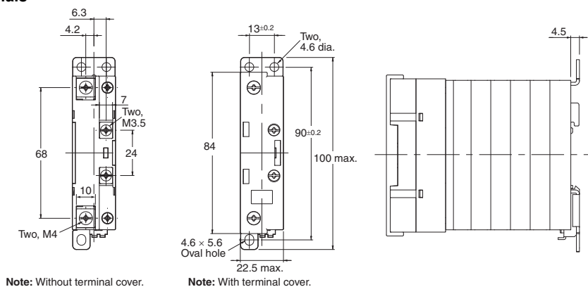
Mounting Holes
