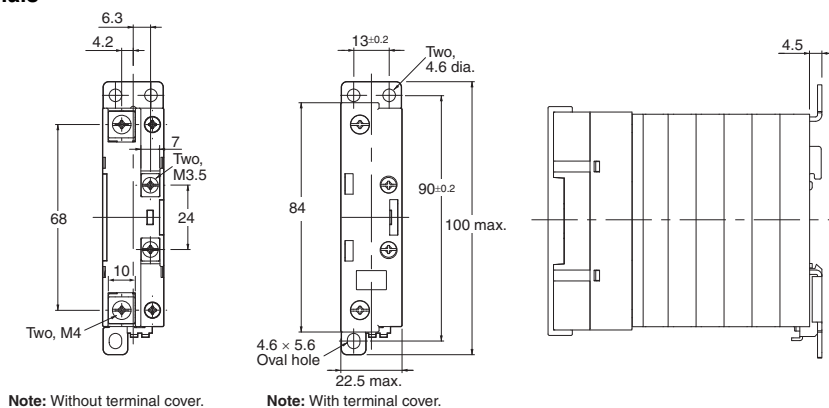
Mounting Holes
