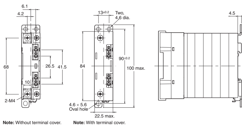
Mounting Holes
