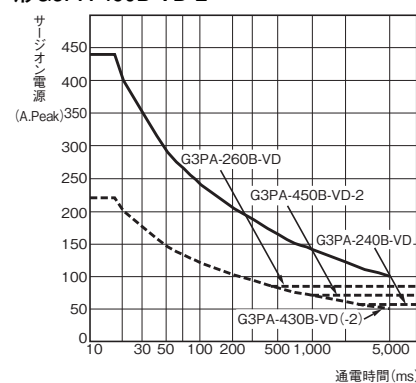
形G3PA-240B-VD、形G3PA-260B-VD、 形G3PA-430B-VD、形G3PA-430B-VD-2、 形G3PA-450B-VD-2
