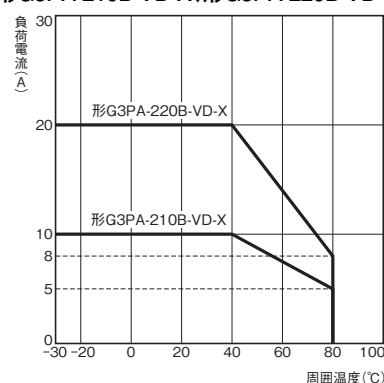
形G3PA-210B-VD-X、形G3PA-220B-VD-X
