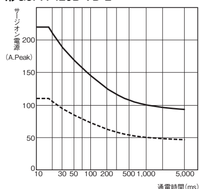
形G3PA-220B-VD-X、 形G3PA-420B-VD、 形G3PA-420B-VD-2
