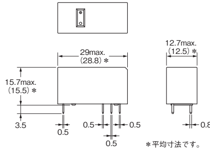
形G2RL-1(-HA、-H、-PW1)
