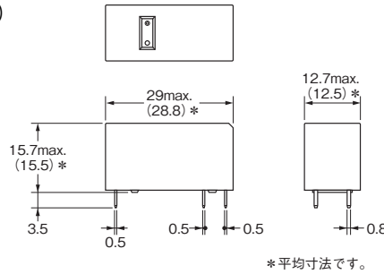
形G2RL-1A-E(-ASI、-HA、-PW1) 形G2RL-1A-E-CV-HA
