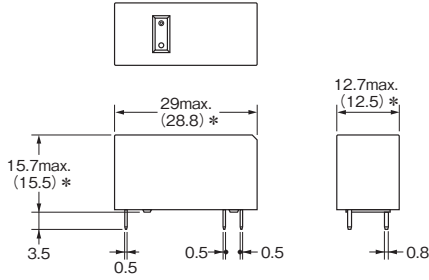
形G2RL-1A(-H、-PW1)
