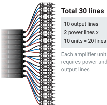
Typical fiber amplifier unit (When connecting 10 channels)
