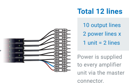
2-channel model E3X-MZV Wire-saving connector model
