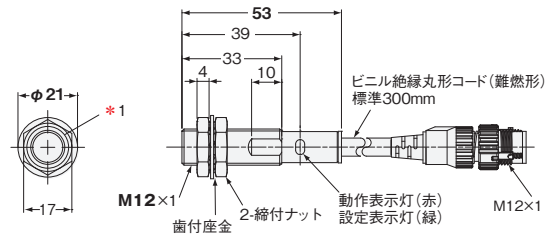
形E2EF-X12D1-M1TGJ -QX12D1-M1TGJ
