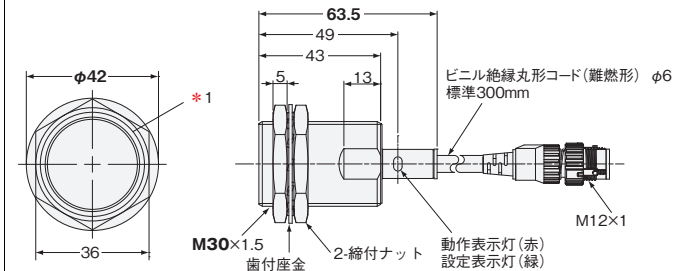
形E2EF-X12D1-M1TGJ -QX12D1-M1TGJ
