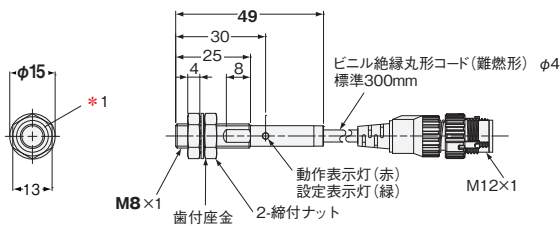
形E2EF-X2D1-M1TGJ -QX2D1-M1TGJ
