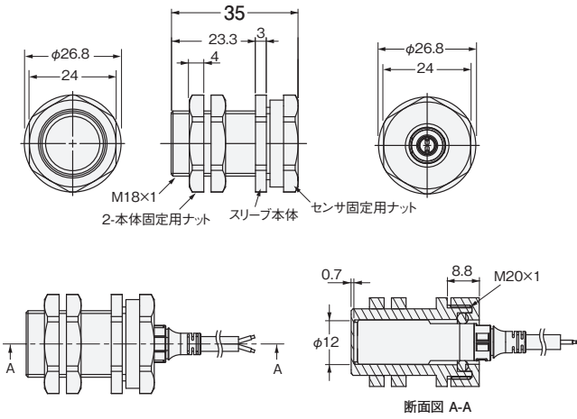
形Y92E-J12S18
