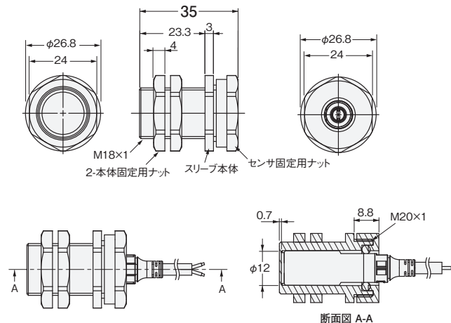
形Y92E-J12S18
