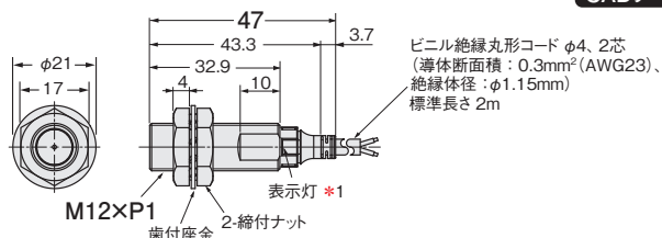
形E2E-X2R5D□
