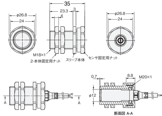
形Y92E-J12S18
