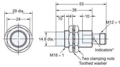
Diagram 14 E2E-X14MD□-M1(G)/E2E-X10ME□-M1/X10MF□-M1
