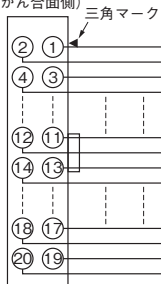
形XG4M-2030-T (かん合面側)
