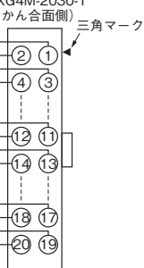
形XG4M-2030-T (かん合面側)
