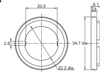
30-dia. Resin Attachment A22Z-A30
