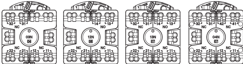
Three contacts (3NC) Three contacts (2NC + 1NO) Four contacts (3NC + 1NO) Four contacts (4NC)
