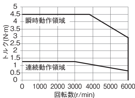
・形R88M-1AL1K530T
