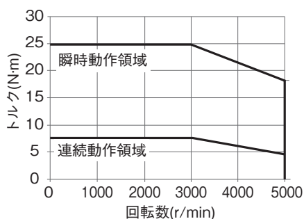
・形R88M-1AL2K630T
