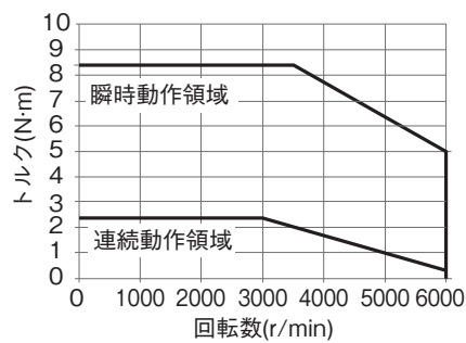
・形R88M-1AL2K030T
