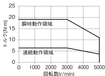
・形R88M-1AL2K030T
