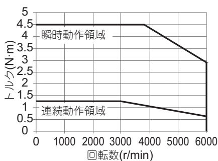
・形R88M-1M40030T
