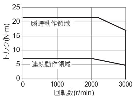
・形R88M-1M1K520C
