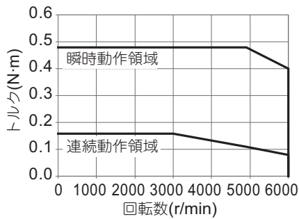
・形R88M-1M05030S
