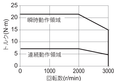
・形R88M-1M1K520T
