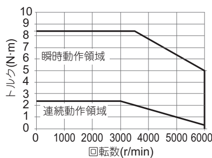
・形R88M-1M75030T
