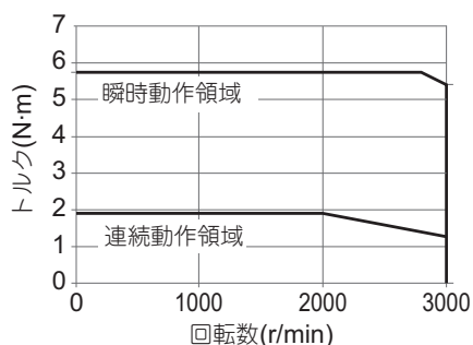
・形R88M-1M40020C
