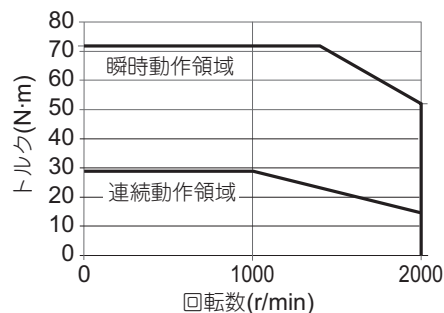
・形R88M-1M3K010C
