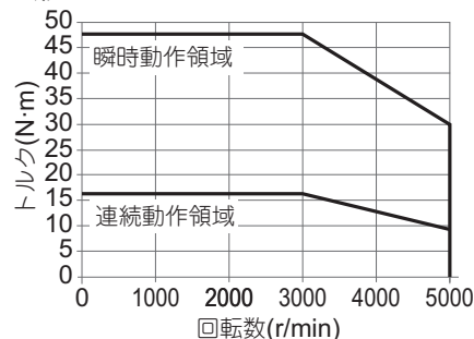
・形R88M-1L5K030C
