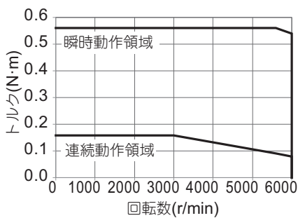
・R88M-1M05030T
