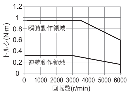
・形R88M-1M10030S
