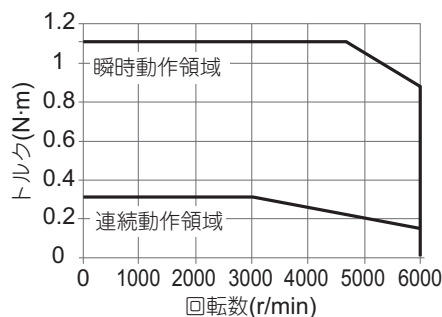
・形R88M-1M10030T
