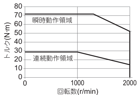
・形R88M-1M3K010C
