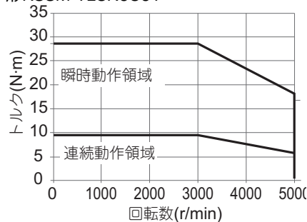
・形R88M-1L3K030T
