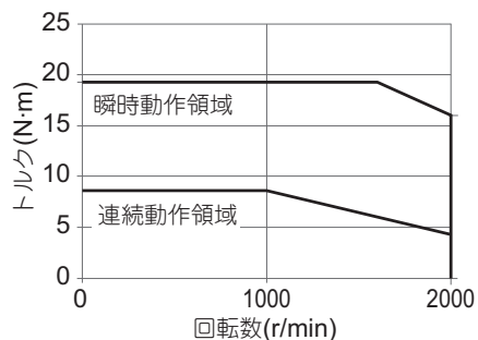
・形R88M-1M90010C
