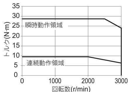
・形R88M-1M2K020T
