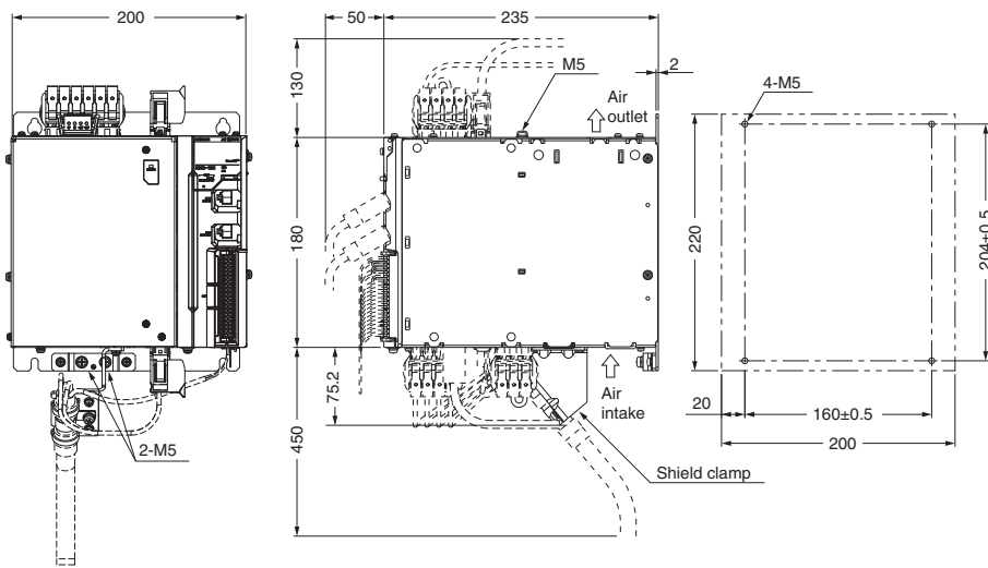
Mounting dimensions
