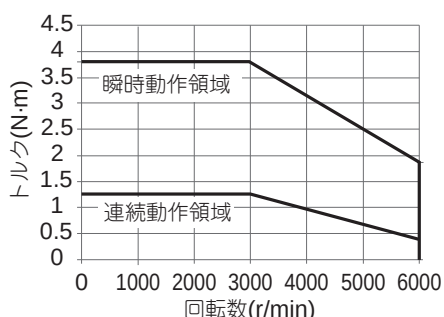
・形R88M-1M40030S
