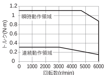
・形R88M-1M10030T
