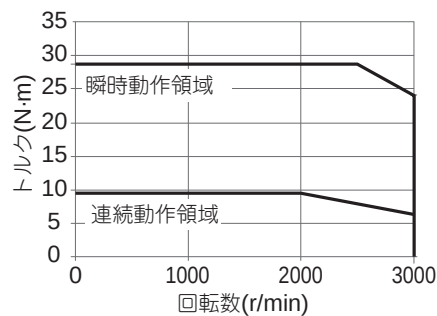
・形R88M-1M2K020T
