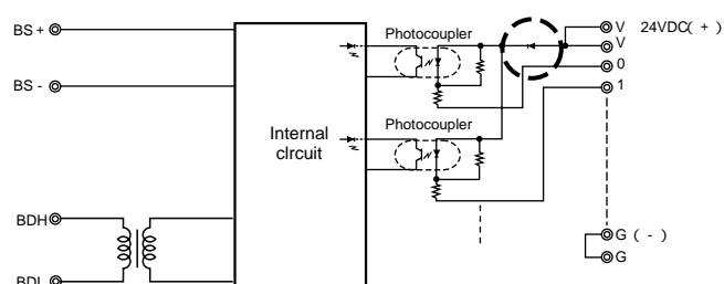
形SRT2-ID08
