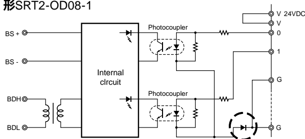
形SRT2-OD08-1
