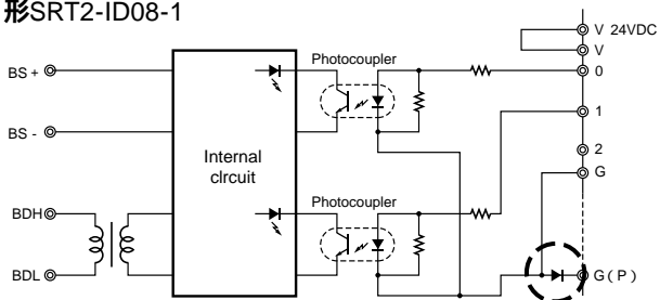
形SRT2-ID08-1
